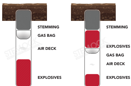
Production Air Deck Blasting with Less Explosives
